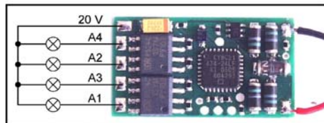
The two connection options for the decoder
